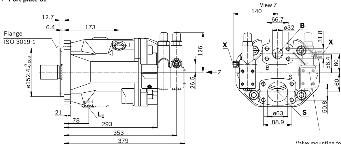
Valve mounting for counter-clockwise rotation
